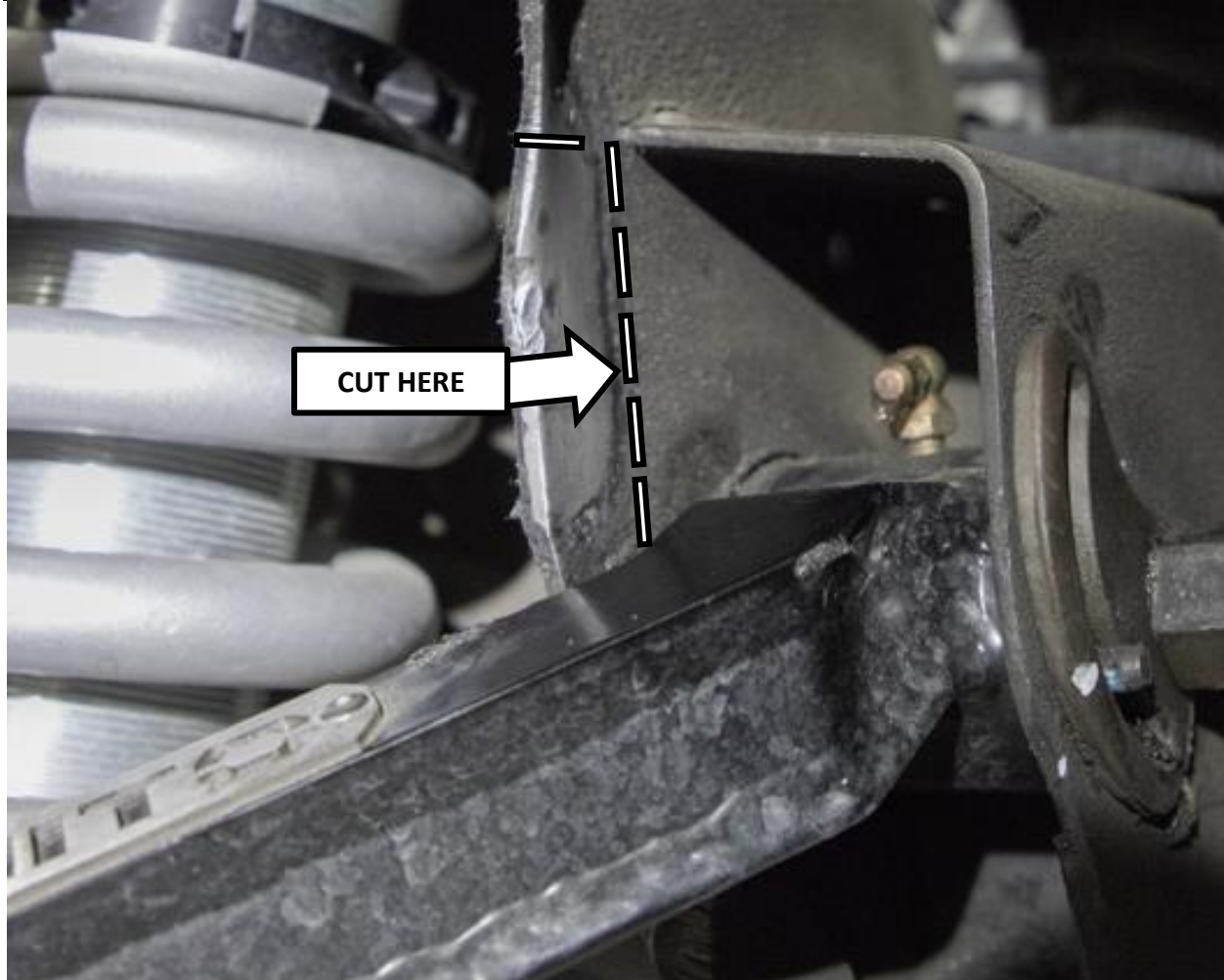
Figure 4: Shock Tower Edge Cut Location
